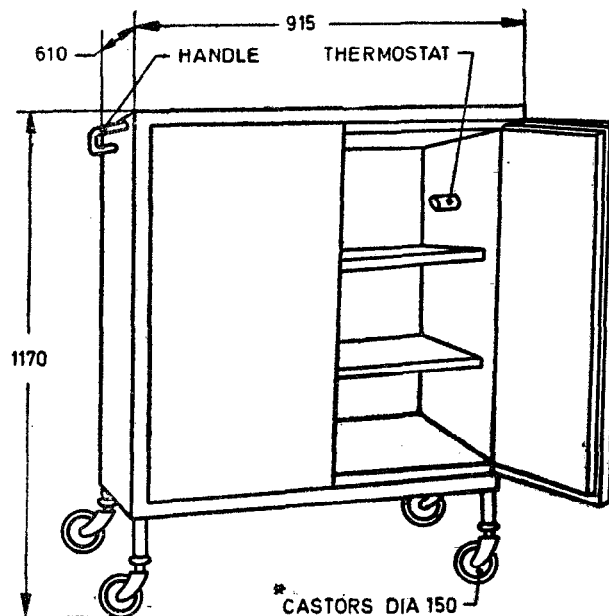
FIG. 1 TROLLEY, HOT FOOD, TRAY TYPE
